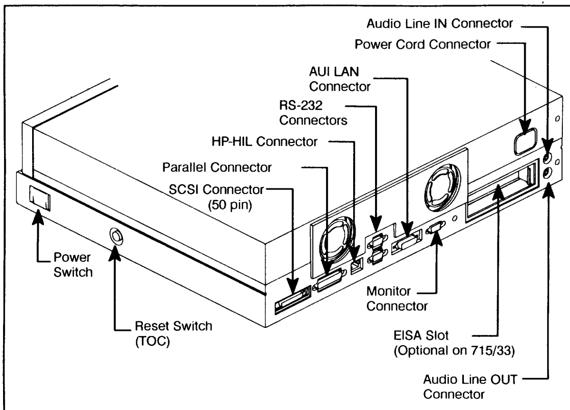
Model 715 Back Panel
